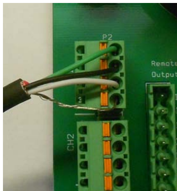
Figure 9A. Connecting Cables to Switch Box for Biaxial Sensor
