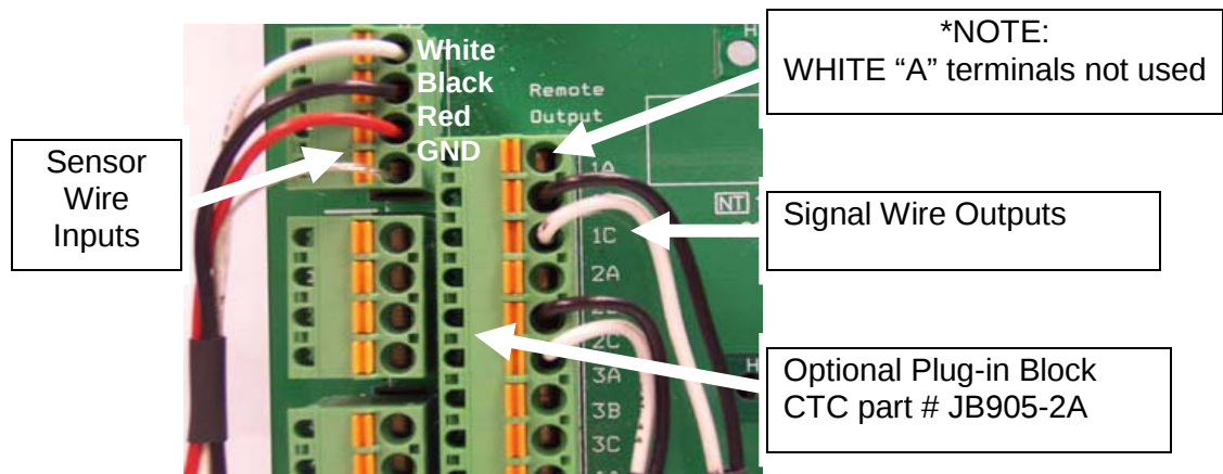
Figure 9B. Optional Plug-in Block #JB905-2A for Vibration and 4-20mA
